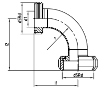
CODO 90° M/T SMS BEND 90° M/N SMS COUDE 90° F/E SMS
