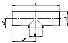
TE SOLDAR CORTA SMS SHORT WELDING TEE SMS TE COURTE A SOUDER SMS
